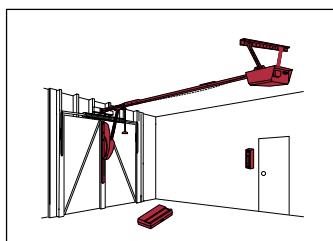
927-756 4410EGB-433C Kit for canopy doors (includes canopy door converter arm)
